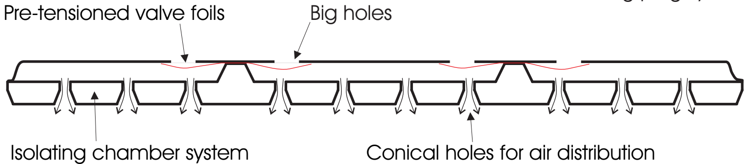
Surrounding plug system
